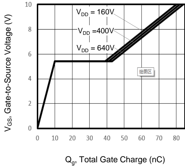
Figure 8. Gate Charge
