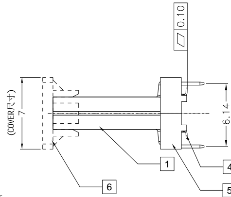
WITHOUT COVER
