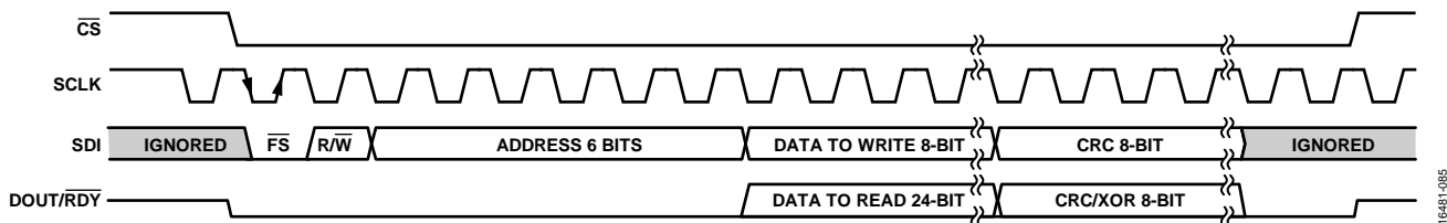
Figure 89. Data Output Format When Using CRC
