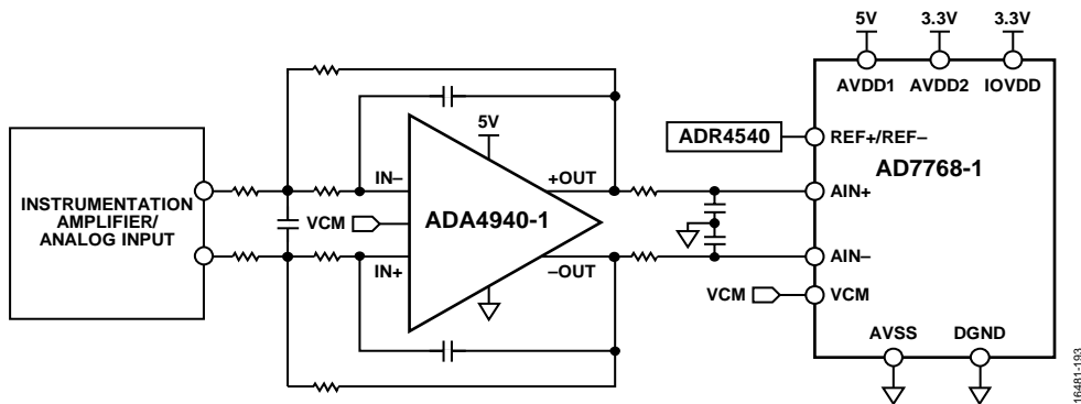
Figure 97. Implementation of a Multiple Feedback, Low-Pass Filter
