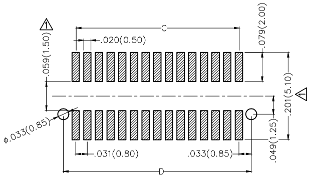
Recommended P.C.Board Layout General Tolerances: ±0.05mm
