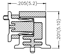
Mating Section
