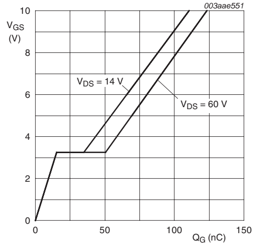
T_j = 25^\circ\text{C}; I_D = 25\text{ A} Fig 14. Gate-source voltage as a function of gate charge; typical values
