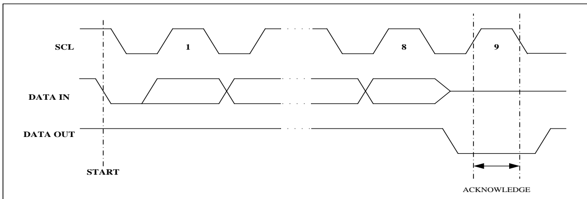
Figure 3. Output Acknowledge
