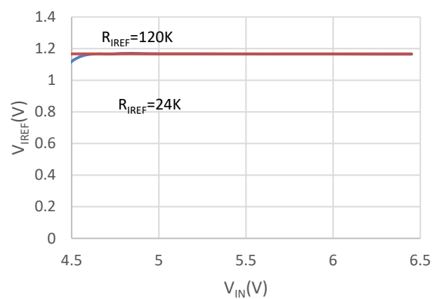
V_{\text{IREF}} vs V_{\text{IN}}
