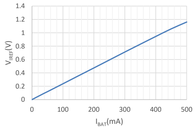
V_{\text{IREF}} vs I_{\text{BAT}}
