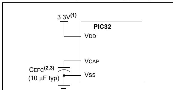
FIGURE 27-1: CONNECTIONS FOR THE ON-CHIP REGULATOR
