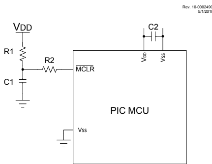
Figure 2-1. Recommended Minimum Connections
