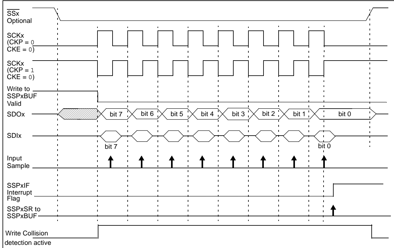
FIGURE 15-9: SPI MODE WAVEFORM (SLAVE MODE WITH CKE = 0)
