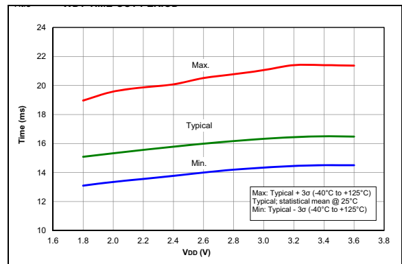
FIGURE 29-46: WDT Time-Out Period, PIC12LF1612/16F1613 Only.
