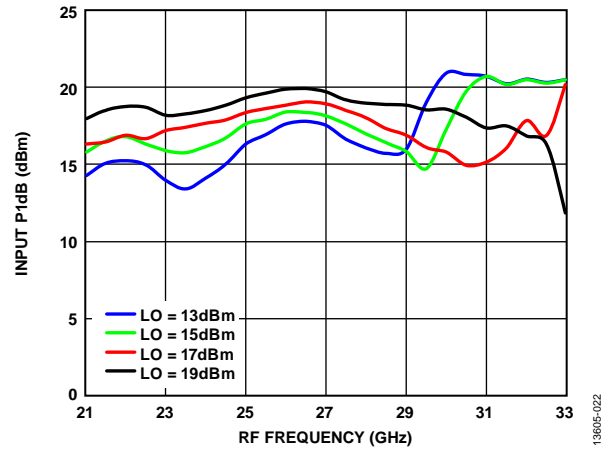
Figure 24 Input P1dB vs. RF Frequency at Various LO Powers, TA = 25°C
