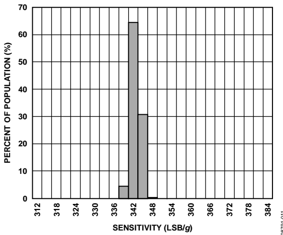
Figure 11. Z-Axis Sensitivity, V_S = V_{DD/IO} = 3.3 V , 25°C
