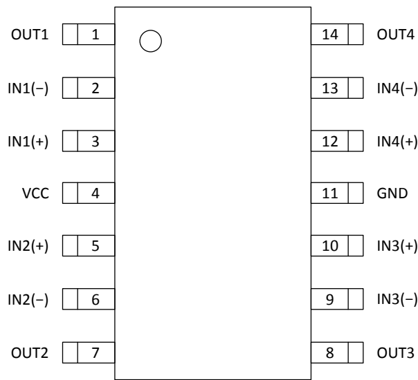
SOP-14
