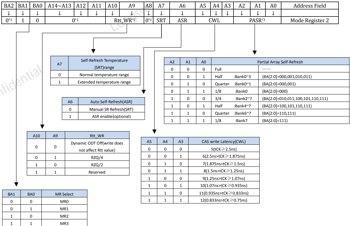
Figure 12 MR2 Programming
