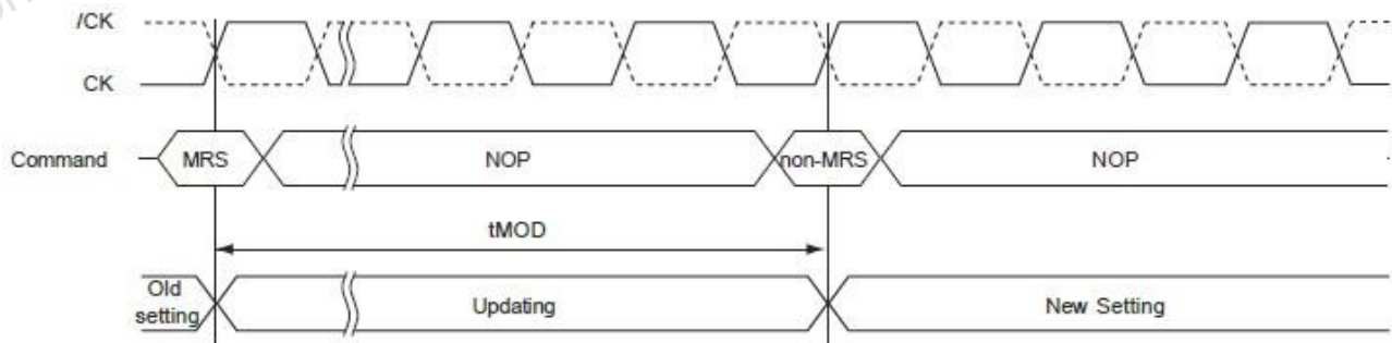
Figure 9 t_{MOD} Timing
