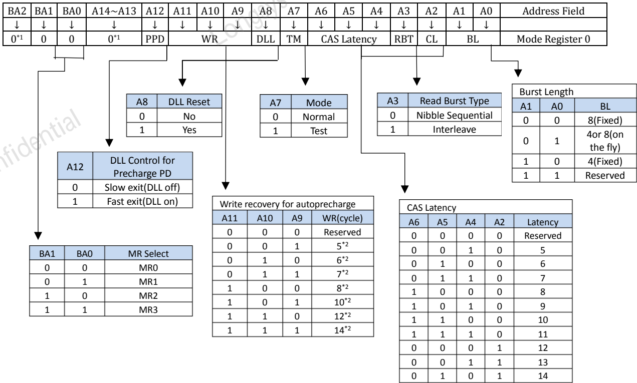
Figure 10 MR0 Programming
