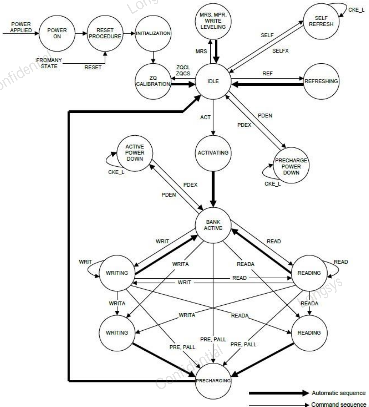
Figure 6 State Diagram
