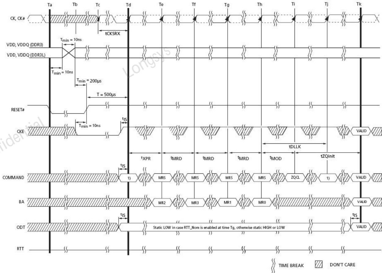
Figure 7 Reset Procedure at Power Stable Condition
