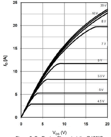
Figure 2: On-Region Characteristics@125°C
