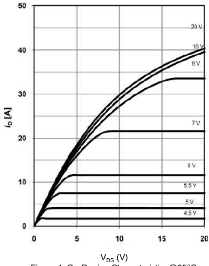
Figure 1: On-Region Characteristics@25°C
