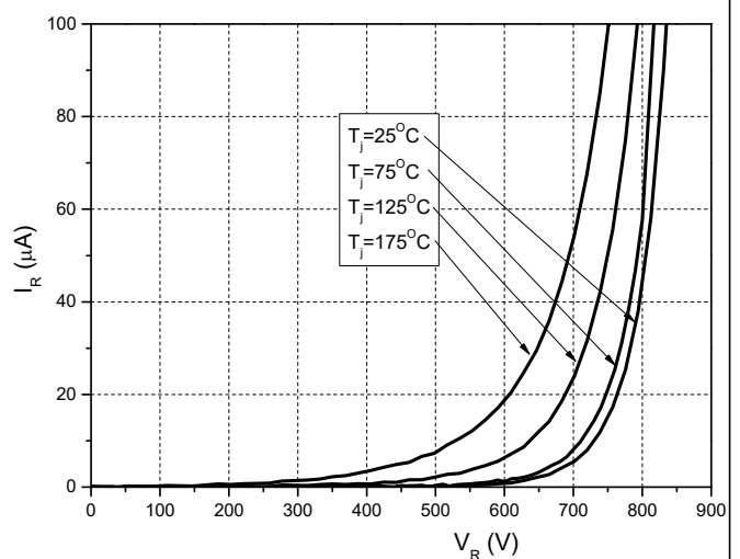
Figure 2. Reverse Characteristics
