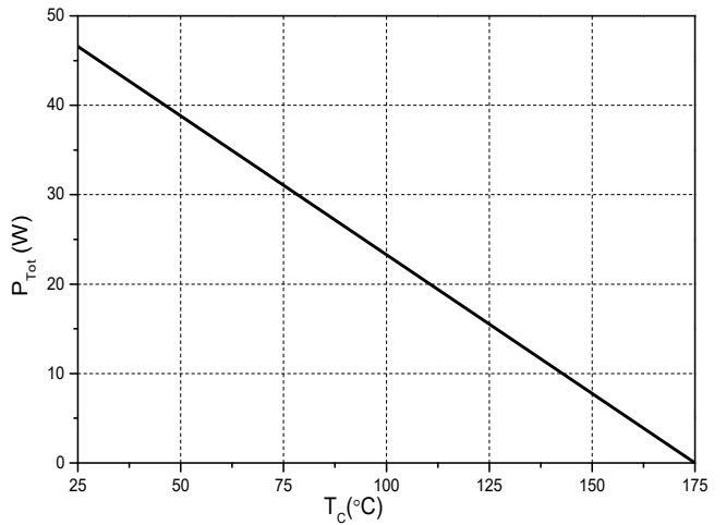
Figure 6. Power Derating
