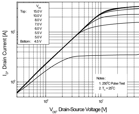
Figure 1. On-Region Characteristics
