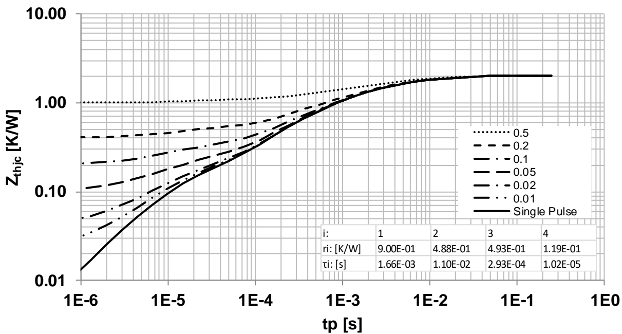
Figure 21 Max. transient thermal resistance (MOSFET/diode) (Z_{th(j-c,max)} = f(t_p), \text{ parameter } D = t_p/T, \text{ thermal equivalent circuit in Fig. D})
