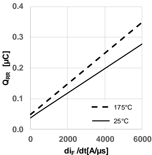
Figure 19 Typical reverse recovery charge as a function of diode current slope ( Q_{rr} = f(di_i/dt) , V_{DD} = 800V , V_{GS} = 0V/18V , I_D = 4A , ind. load, test circuit in Fig.E, body diode at V_{GS} = 0V )
