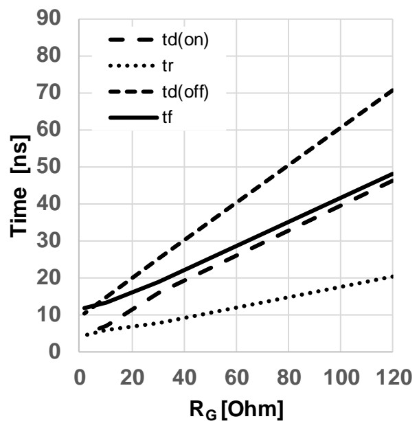
Figure 18 Typical switching times as a function of gate resistor ( t = f(R_{G,ext}) , V_{DD} = 800V , V_{GS} = 0V/18V , I_D = 6A , T_{vj} = 175^{\circ}C , ind. load, test circuit in Fig. E, diode: body diode at V_{GS} = 0V )
