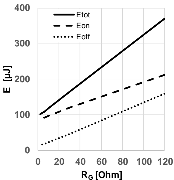
Figure 17 Typical switching energy losses as a function of gate resistance ( E = f(R_{G,ext}) , V_{DD} = 800V , V_{GS} = 0V/18V , I_D = 6A , T_{vj} = 175^{\circ}C , ind. load, test circuit in Fig. E, diode: body diode at V_{GS} = 0V )
