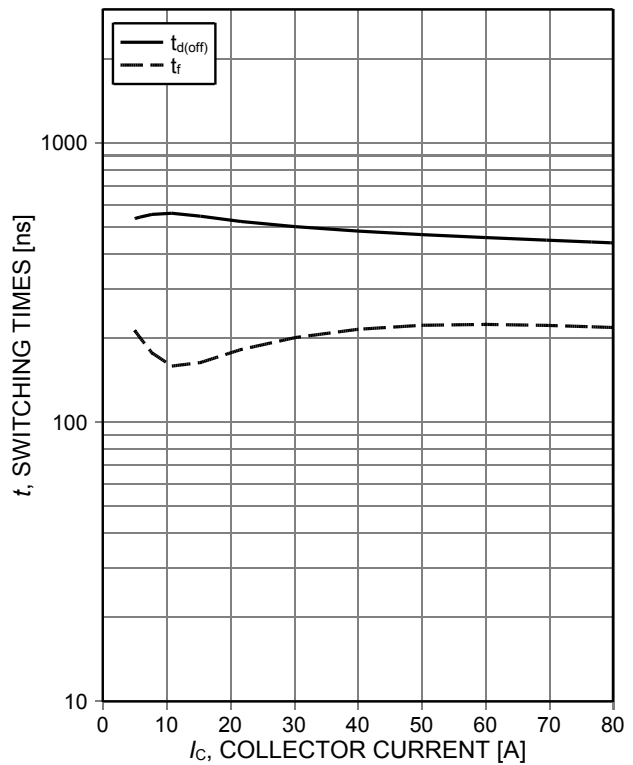
Figure 8. Typical switching times as a function of collector current (inductive load, T_{vj}=175^{\circ}C , V_{CE}=600V , V_{GE}=0/15V , r_G=10\Omega , Dynamic test circuit in Figure E)
