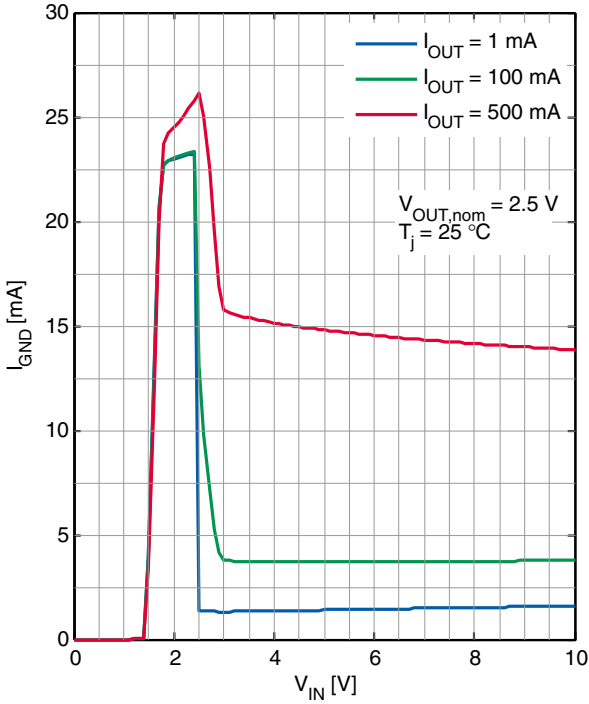
GND Pin Current I_{GND} versus Input Voltage V_{IN} ( V_{OUT,nom} = 2.5\text{ V} )
