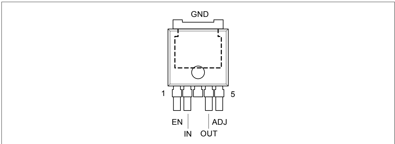
Figure 3 Pin Configuration PG-T0252-5
