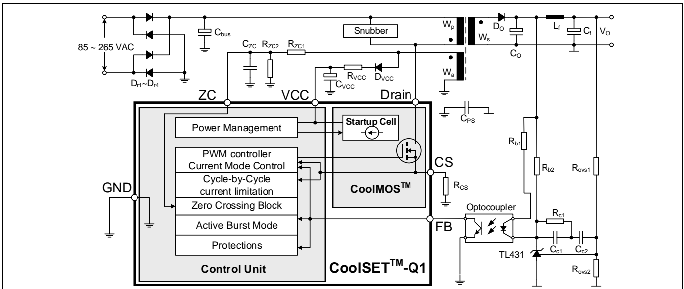
Figure 1 Typical application
