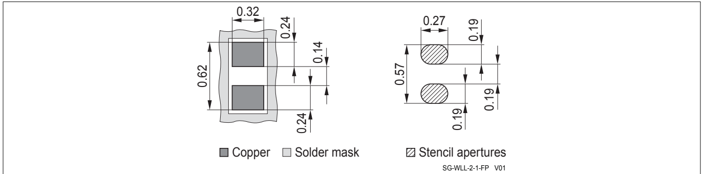
Figure 13 WLL-2-1 footprint
