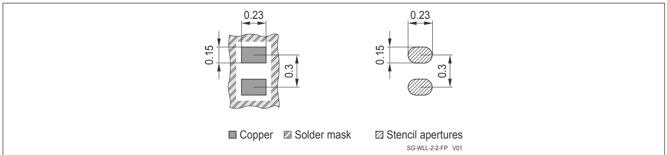
Figure 14 WLL-2-2 footprint
