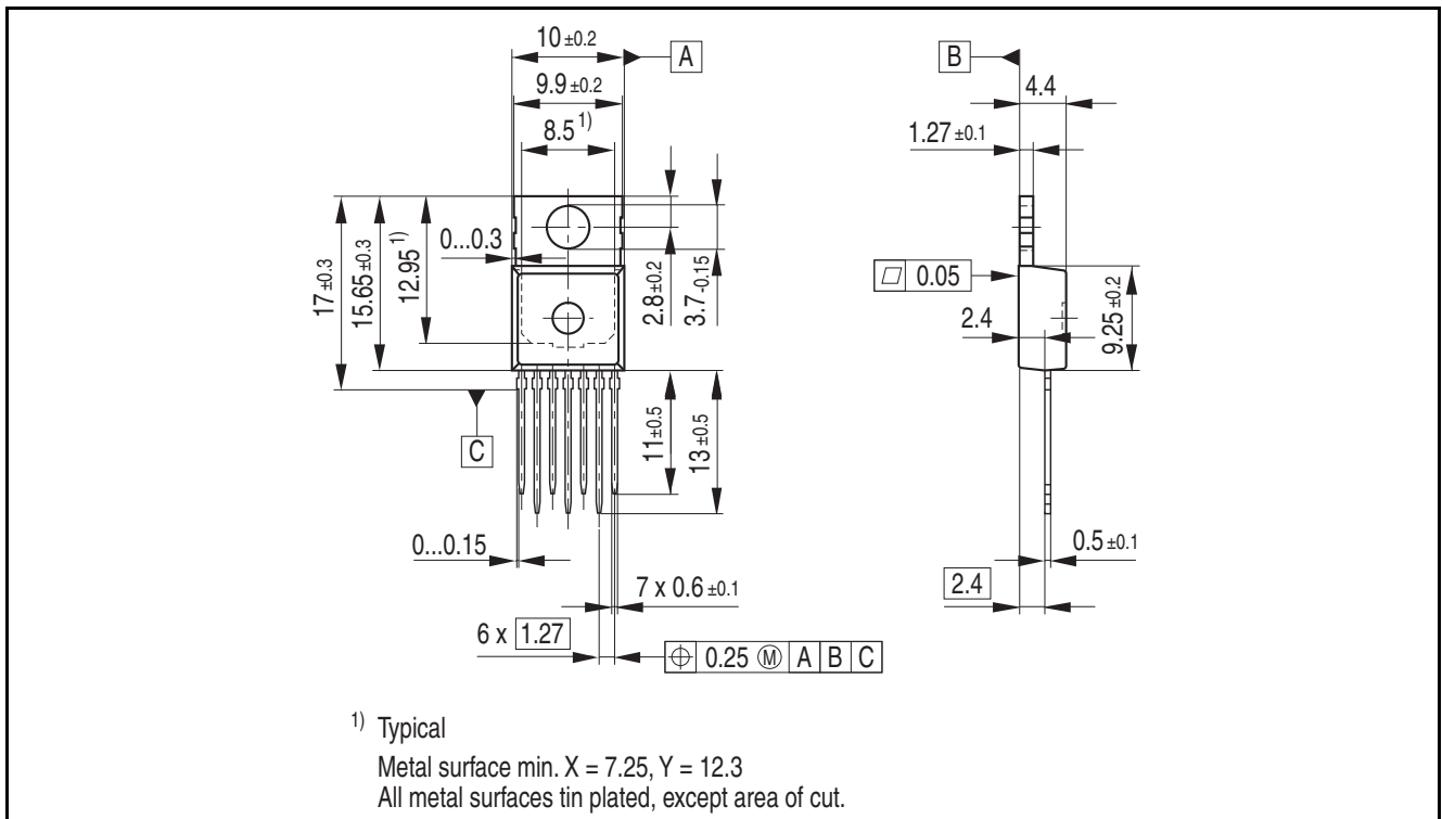
Figure 2 PG-TO220-7-12
