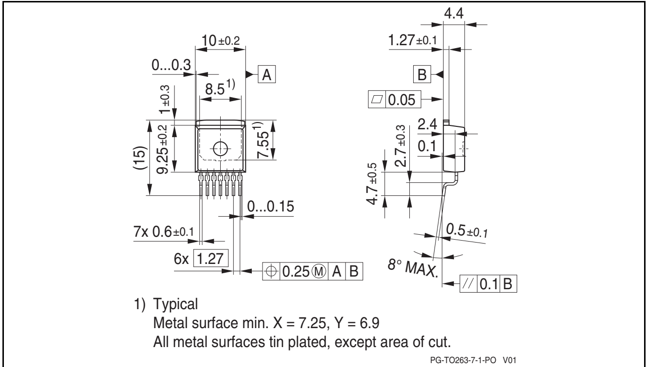
Figure 1 PG-TO263-7-1
