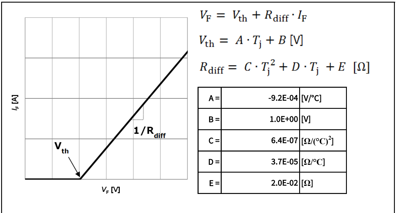
Figure 6 Simplified forward characteristics model V_F = f(I_F) ; -40°C < T_j < 175°C; I_F < 40 \text{ A}
