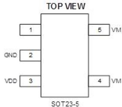
Figure 2. Pin Configuration
