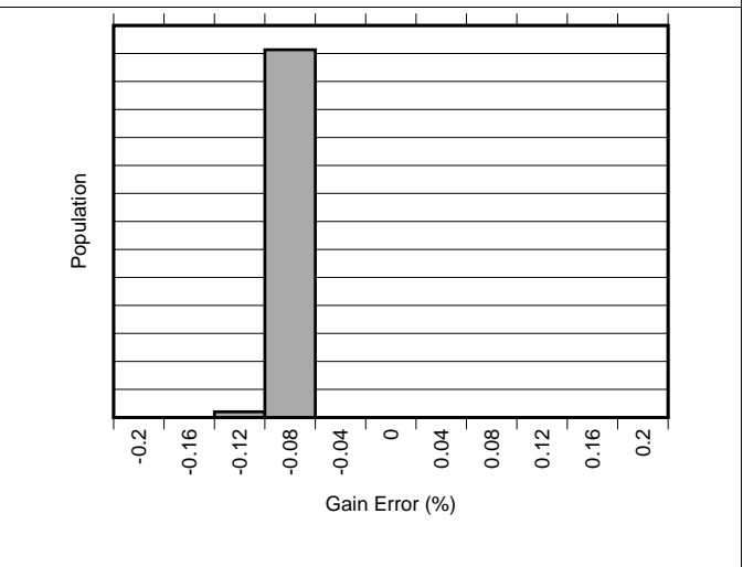
Figure 12. Gain Error Distribution (INA301A3-Q1)
