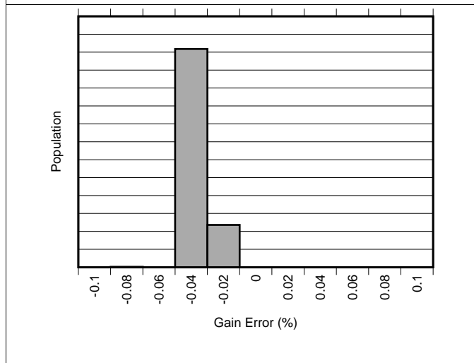
Figure 11. Gain Error Distribution (INA301A2-Q1)
