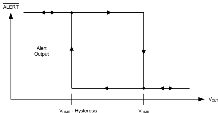
Figure 37. Typical Comparator Hysteresis
