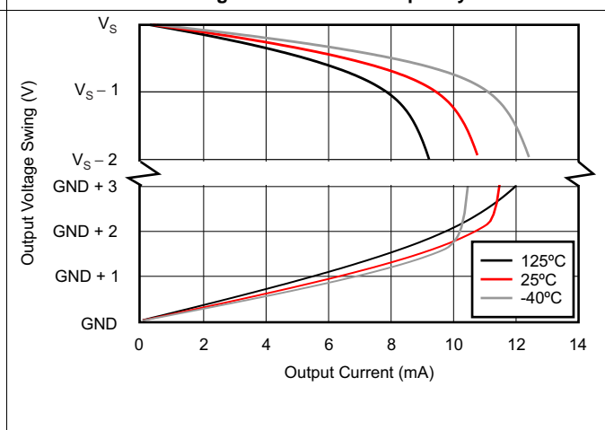
Figure 16. Output Voltage Swing vs Output Current
