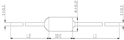
L1=34mm±3mm, L2=20mm±3mm or 34mm±3mm. The length will be customized according to customer needs.
