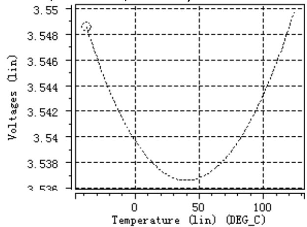
Output Voltage vs. Temperature (Cin=1.0uF,Cout=1.0uF,Iout=1mA)
