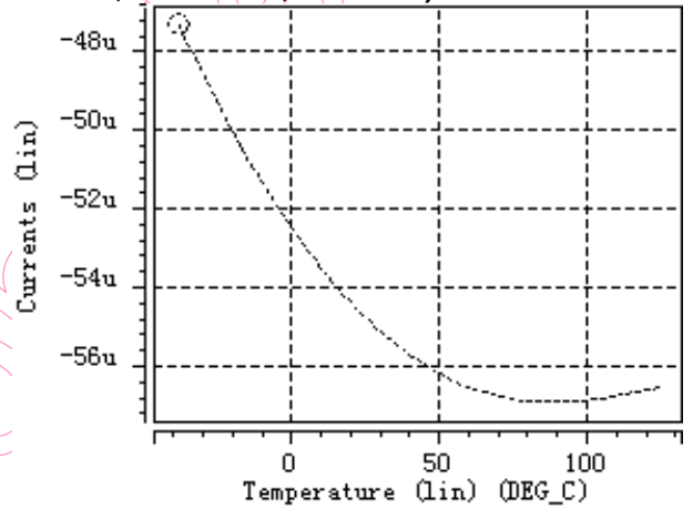
Supply Current vs. Temperature (Cin=1.0uF,Cout=1.0uF,Iout=0mA)
