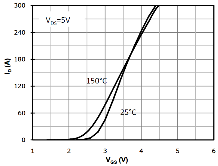
Fig 2: Transfer Characteristics
