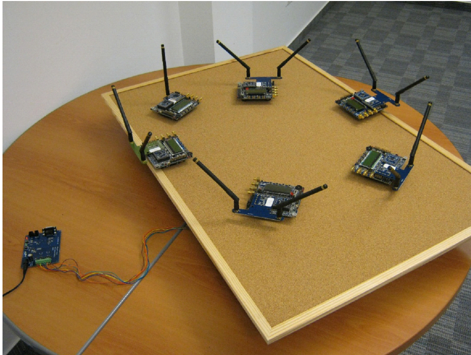
Figure 11. Measurement Setup with Turntable (Artificial Fading Simulator)
