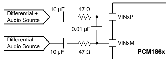
图 63. Differential Input Circuit With Additional AntiAliasing Filter
