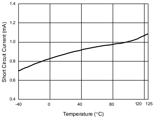
Fig. 7 Short Circuit Current (mA) vs. Temperature
