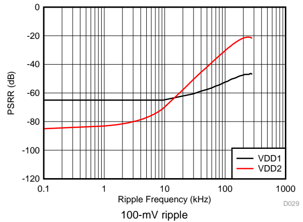
Figure 32. Power-Supply Rejection Ratio vs Ripple Frequency 100-mV ripple
