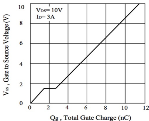
Figure 6. Gate Charge
