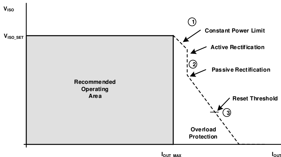
Figure 27. V_{ISO} Load Recommended Operating Area Description
