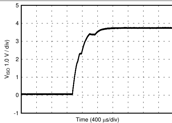
Figure 50. V_{ISO} Soft Start at 90% Rated Load, 5.0-V Input, 3.7-V Output
