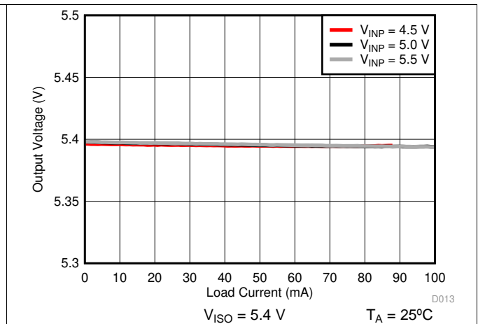
Figure 17. Isolated Supply Voltage ( V_{ISO} ) vs Load Current ( I_{iso} )
