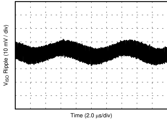
V_{INP} = 5.0\text{ V} V_{ISO} = 3.3\text{ V} Bandwidth = 20 MHz
