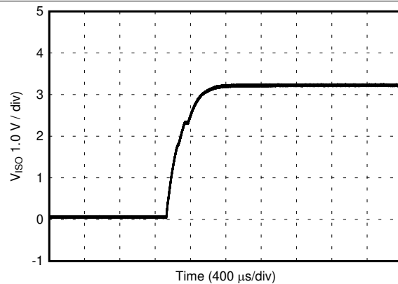
Figure 52. V_{ISO} Soft Start at 90% Rated Load, 5.0-V Input, 3.3-V Output
