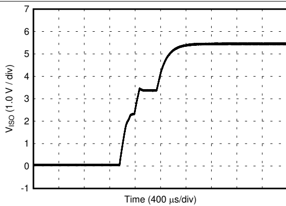
Figure 45. V_{ISO} Soft Start at 10% Rated Load, 5.0-V Input, 5.4-V Output
