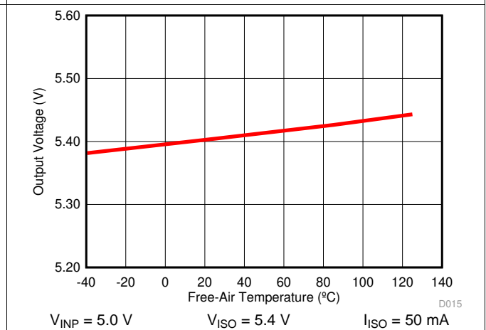
Figure 21. Isolated Supply Voltage ( V_{ISO} ) vs Free-Air Temperature
