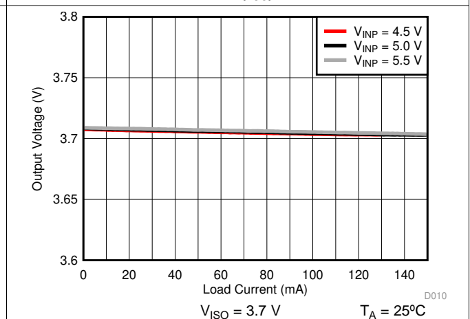
Figure 19. Isolated Supply Voltage ( V_{ISO} ) vs Load Current ( I_{iso} )
