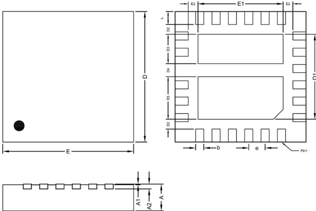
QFN4X4-23 Package
