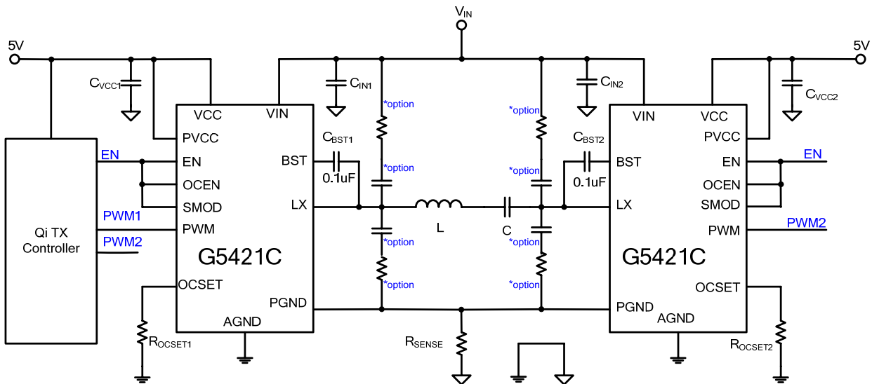
Fig. 4 Application Circuit
