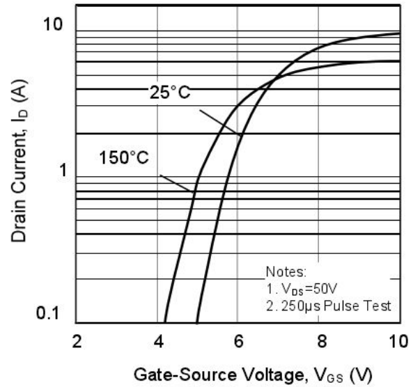
Transfer Characteristics
