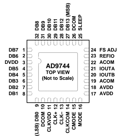
Figure 4. 32-Lead LFCSP
