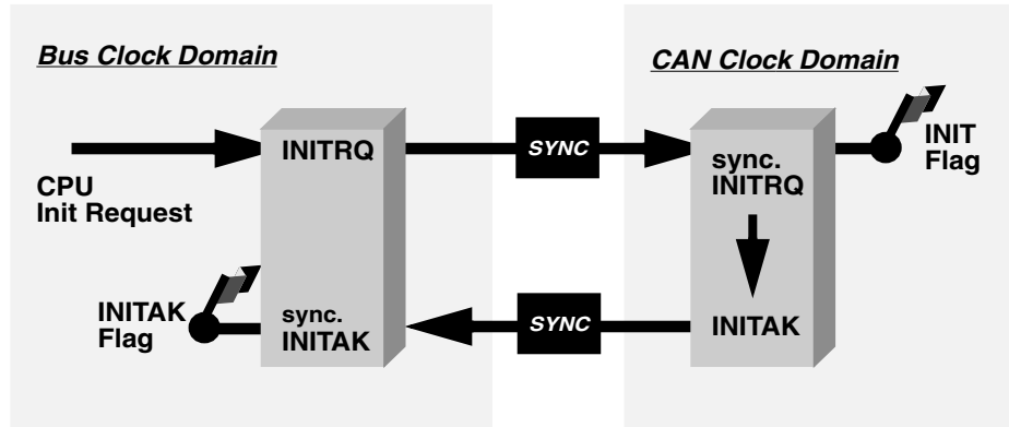
Figure 16-45. Initialization Request/Acknowledge Cycle
