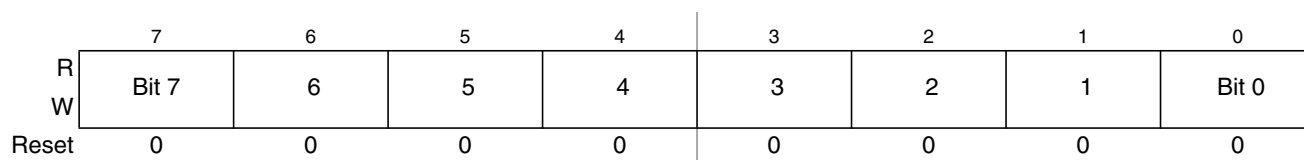
Figure 19-10. PWM Scale A Register (PWMSCLA)
