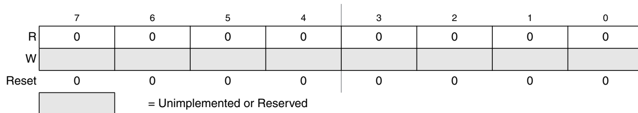
Figure 28-24. Flash Reserved6 Register (FRSV6)
