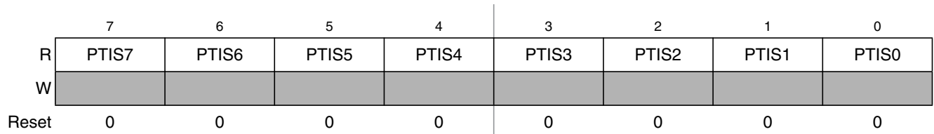
Figure 2-22. Port S Input Register (PTIS)
