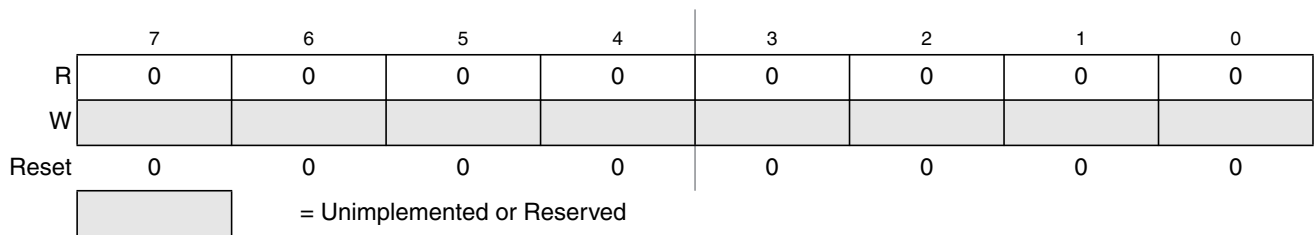
Figure 30-21. Flash Reserved4 Register (FRSV4)
