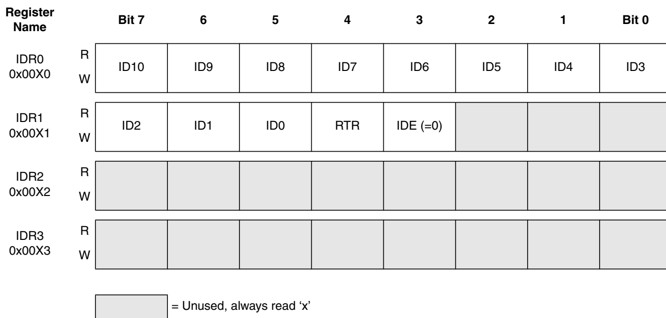
Figure 18-25. Receive/Transmit Message Buffer — Standard Identifier Mapping
