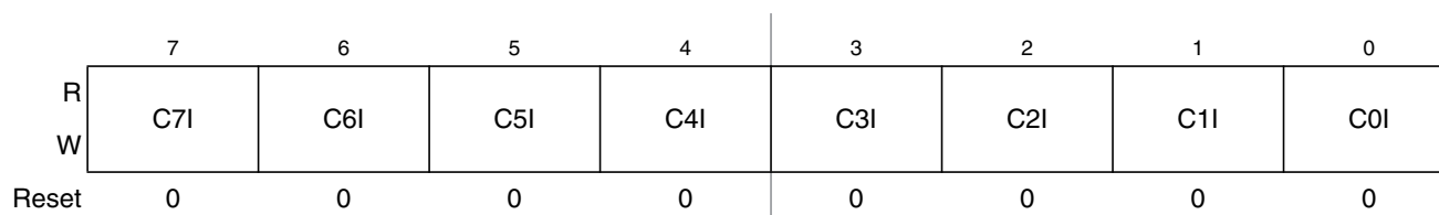
Figure 23-18. Timer Interrupt Enable Register (TIE)
