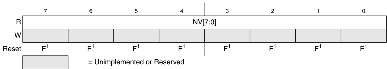
Figure 30-22. Flash Option Register (FOPT)
