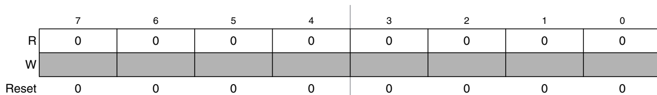
Figure 2-7. Port D Data Register (PORTD)
