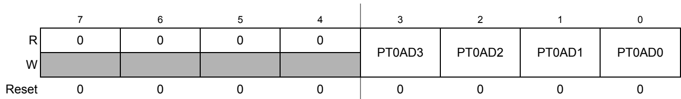
Figure 2-49. Port AD Data Register (PT0AD)
