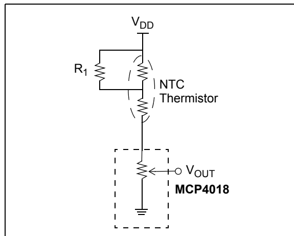
FIGURE 8-6: Thermistor Calibration using a Digital Potentiometer in a Potentiometer Configuration.
