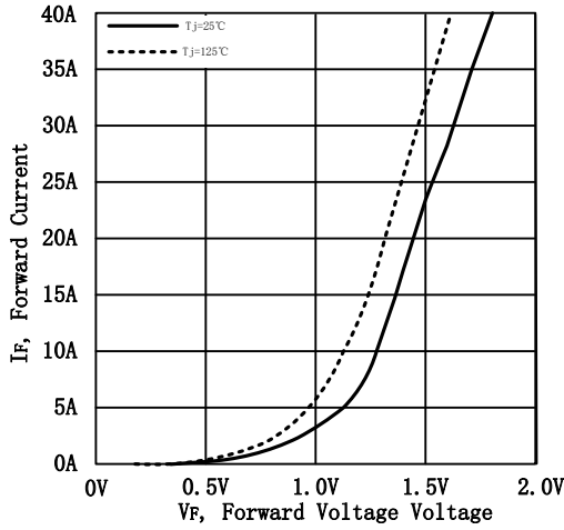
Figure 7 Forward Characteristics
