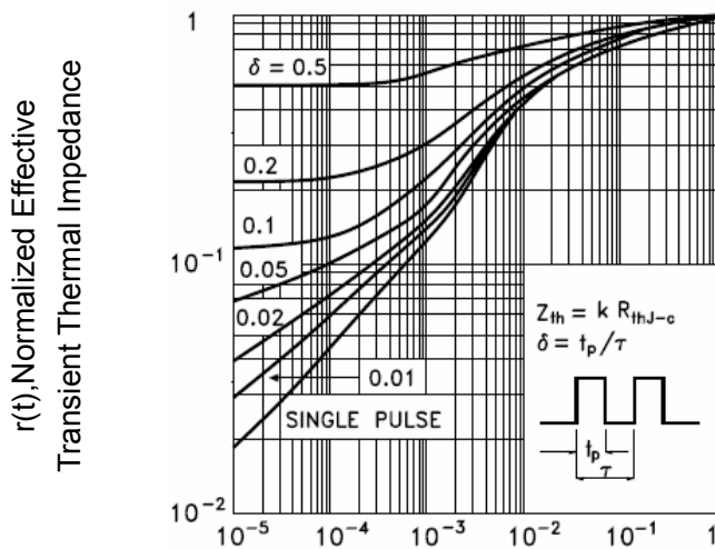
Square Wave Pluse Duration(sec) Figure 11 Normalized Maximum Transient Thermal Impedance
