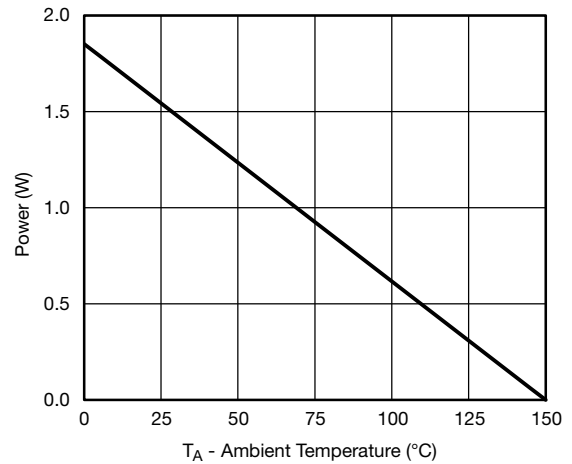
Power, Junction-to-Ambient
