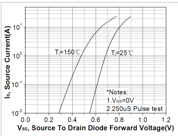
Fig 9. Forward characteristics of reverse diode
